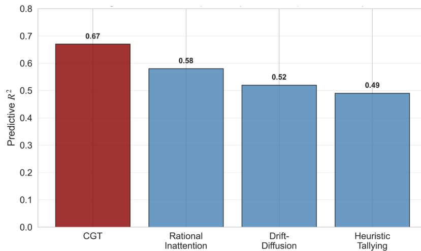
Fig. 3. Hierarchical Bayesian integration. Parameters show narrow credible intervals ( \hat{R} \leq 1.02 ). CGT outperforms benchmarks ( R^2 = 0.67 vs. 0.49–0.58).
