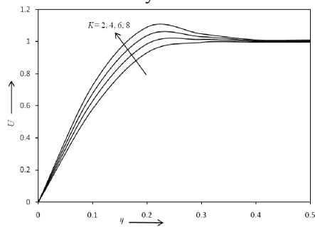
Fig. (5.4). Velocity distribution for different values of k at Gr/Re^2=0.1 & \xi=1
