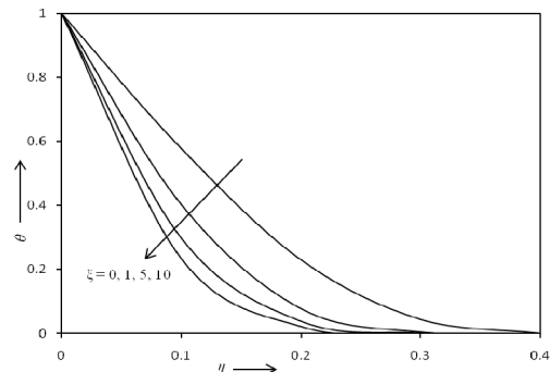
Fig. (5.5). Temperature distribution for different values of \xi at Gr/Re^2=0.1
