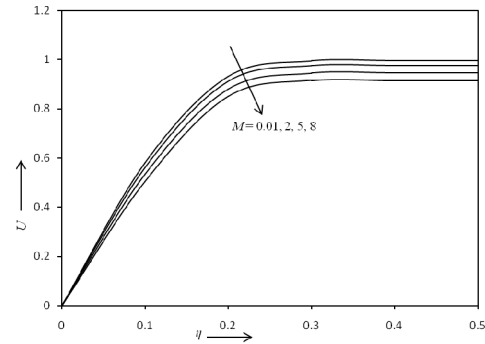
Fig. (5.3). Velocity distribution for different values of M at Gr/Re^2=0.1 & \xi=1
