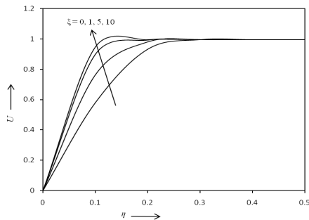
Fig. - (5.1): Velocity distribution for different values of \xi at Gr/Re^2 = 0.1 .
