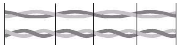
Fig. 5. Why c = f * \lambda
