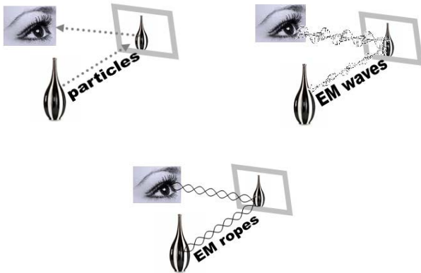
Fig. 10. Reflection: One-way particles and waves versus the interconnecting EM rope.
