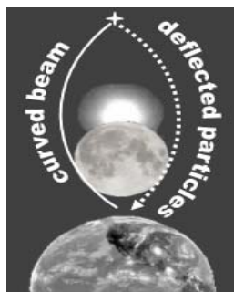
Fig. 7. Does warped space bend or deflect light?
