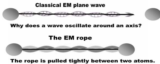
Fig. 6. Why does a plane wave oscillate around an axis? What compels it to travel rectilinearly?
