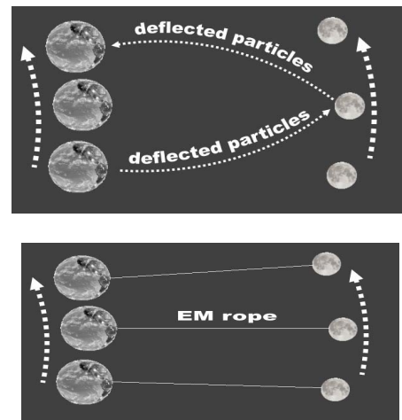
Figs. 8 and 9. The discrete particle and rope versions of the Lunar Ranging Experiment. (For simplicity, only one interconnecting rope is shown.) One-way entities such as particles, waves and wave-packets cannot justify the Principle of Ray Reversibility.. This optical phenomenon can only be justified by a two-way mechanism.
