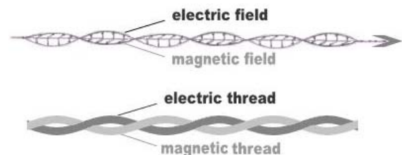
Fig. 1. Wave vs. Rope
