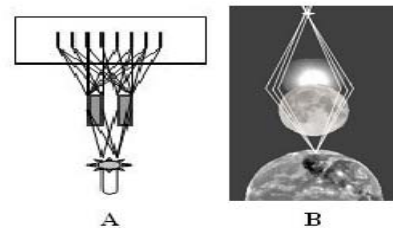
Fig. 12. A. Slit Experiment. B. Gravitational Lensing
