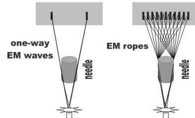
Fig. 11. Needle Experiment: one-way waves vs. interconnecting ropes.
