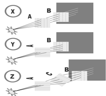
Fig. 16.X: Polarized light. Y: Beam Extinction.
