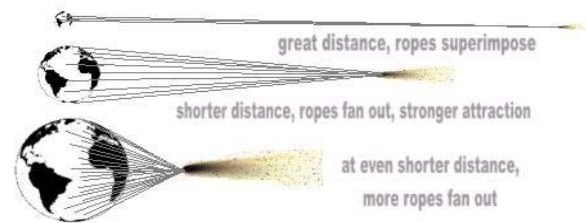
Fig. 17. Action-at-a-distance mediated by EM ropes. At great distances, the ropes superimpose and act as one. At short distances, the ropes fan out and act individually, compelling the comet to accelerate towards Earth.
