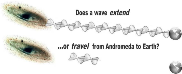
Fig. 2. Does an EM wave extend or travel ?
